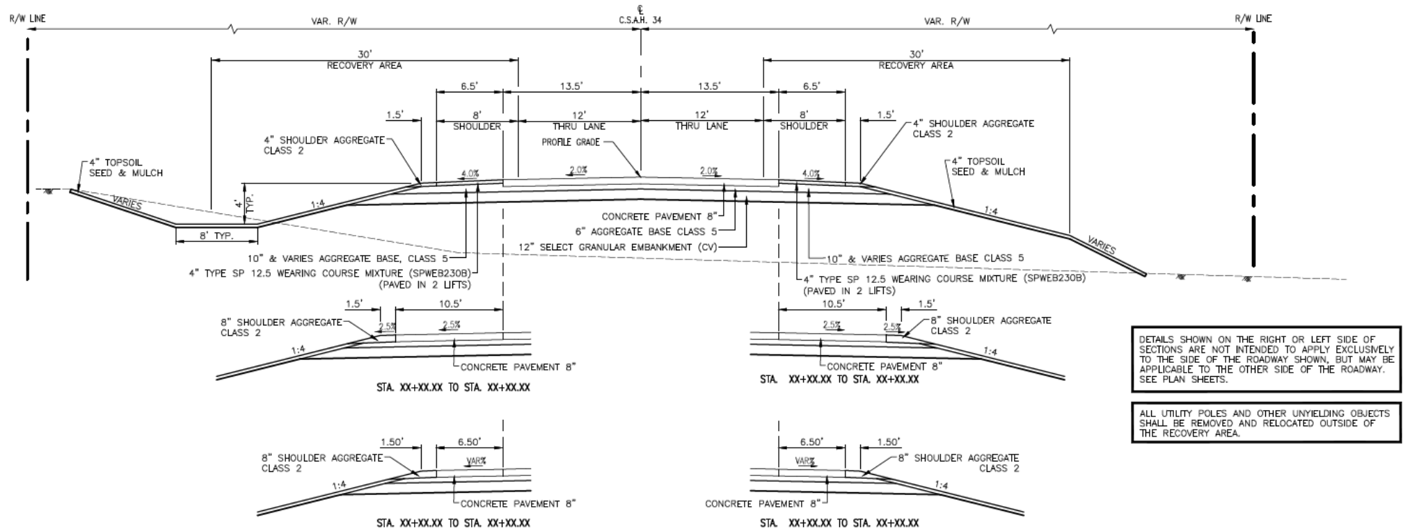
C.S.A.H. 34 TYPICAL SECTION STA. XX+XX.XX TO STA. XX+XX.XX
